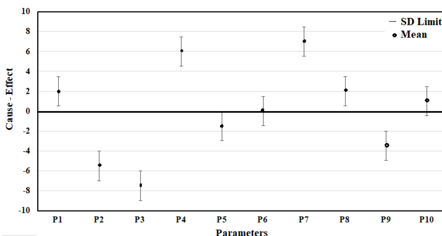
Fig. 11. Mean values and standard deviation limits for subordination of 10 parameters affecting the initial support
