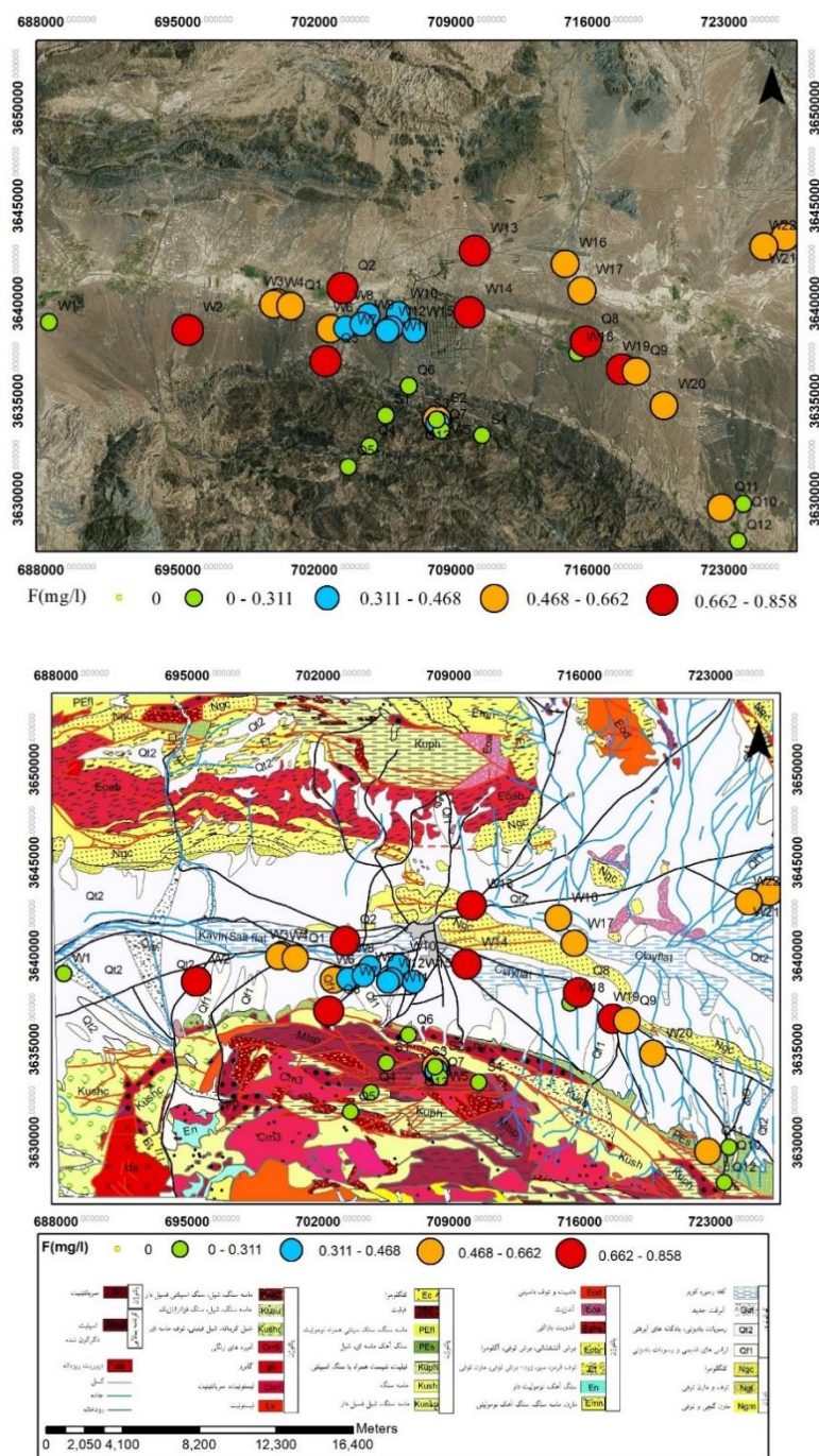
Fig. 17- Fluoride ion dispersion map in the study area
