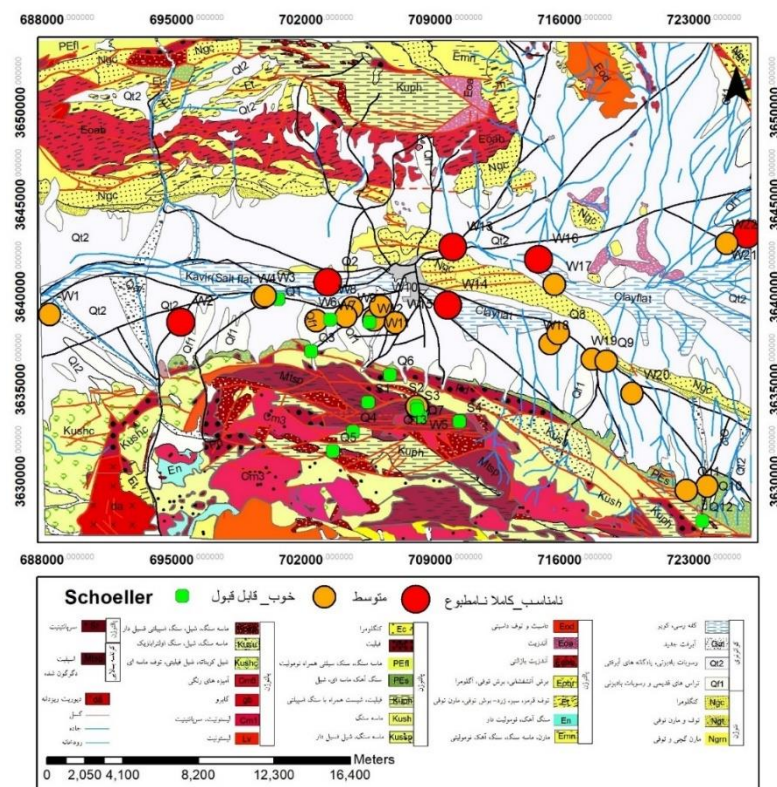
Fig. 10. Distribution of water resources based on Schuler diagram
