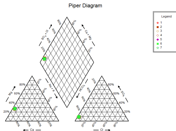
Fig. 3. Piper diagram of Varsakhuran spring water samples
