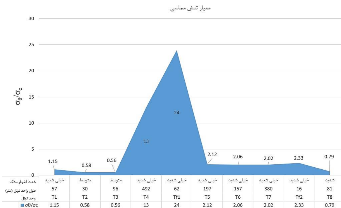
Fig. 3. Evaluation diagram of rock burst intensity based on tangential stress criterion
