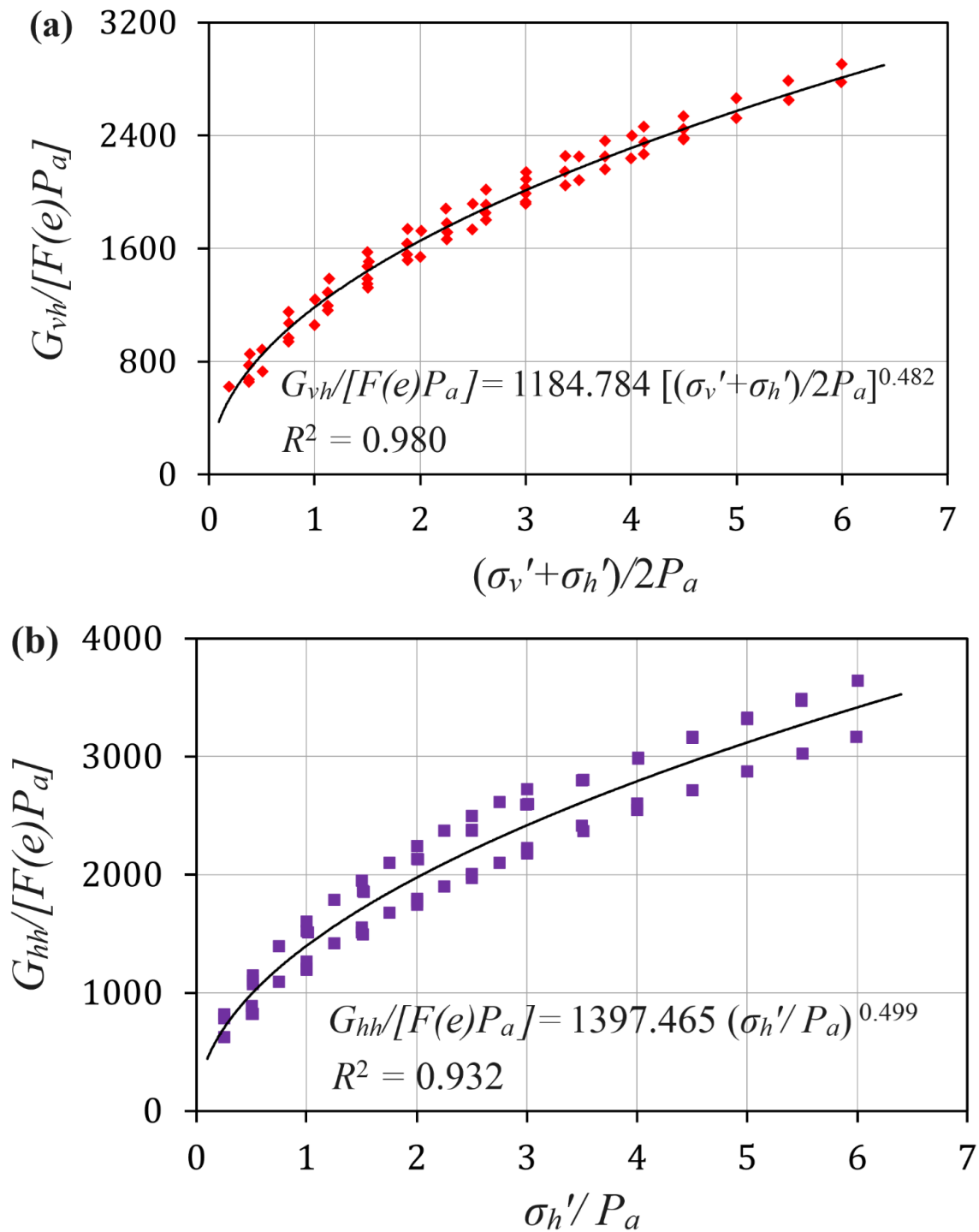
Fig 3. The derivation process of constants A_{vh} and A_{hh} for Kenya sand. (a) Depicting G_{vh}/F(e)P_a versus (\sigma'_v + \sigma'_h)/2P_a for extraction of A_{vh} ; (b) Depicting G_{hh}/F(e)P_a versus \sigma'_h/P_a for extraction of A_{hh}
