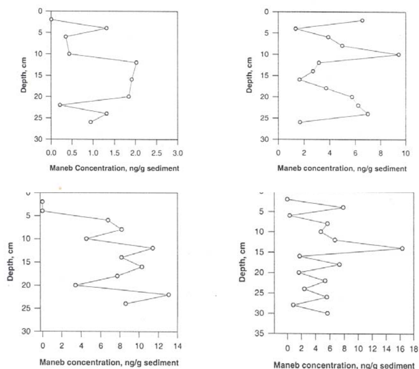
Fig. 8: Distribution of Maneb in the sediments by depth. From top left, clockwise greenfield site, Mostyn Quay site, Pincton Pool site and Mostyn Dock site
