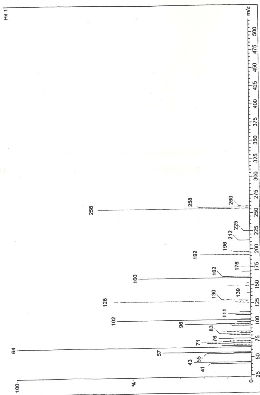
Fig. 7: Mass spectrogram of Maneb
