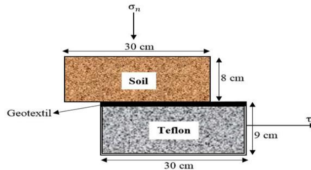
Figure 4. Geotextile position
