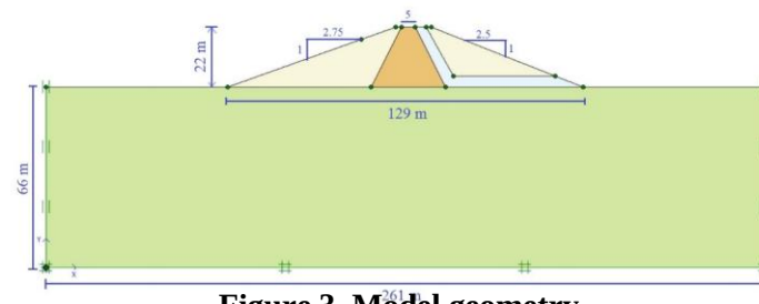
Figure 3. Model geometry
