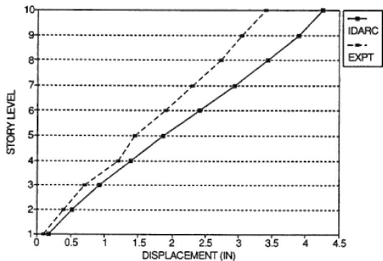
Figure 2. Computed versus observed peak displacement response
