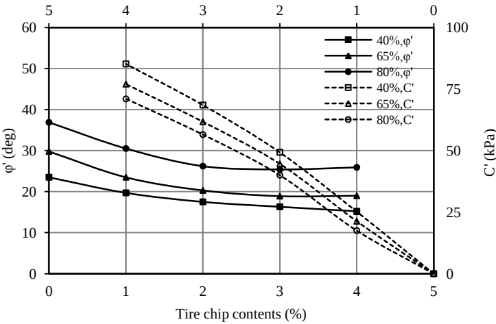
Figure 10. Variation of \phi' and C' with tire chip contents and relative density
